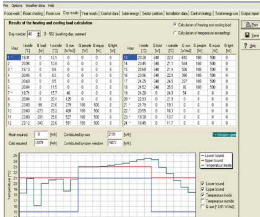
Figure 2. Indoor temperature response when night cooling is applied. Opened windows are indicated by *. The highly fluctuating indoor temperature during night is caused by open/closed control of window opening and the time step of 1 hour. In reality it will be more smooth.
