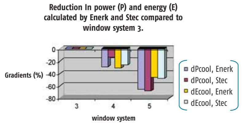
Figure A2 . Reduction in cooling load capacity and energy consumption calculated by two different programs: Enerk and Stc [PhD, Stc]. Both programs show reductions of the same order.
